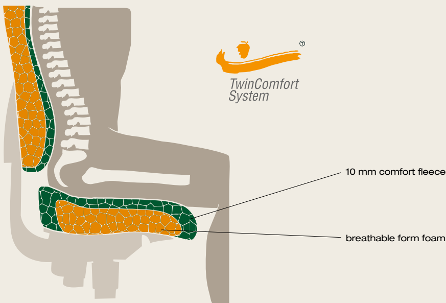
Comfortable double foam seating design (TwinComfort)
